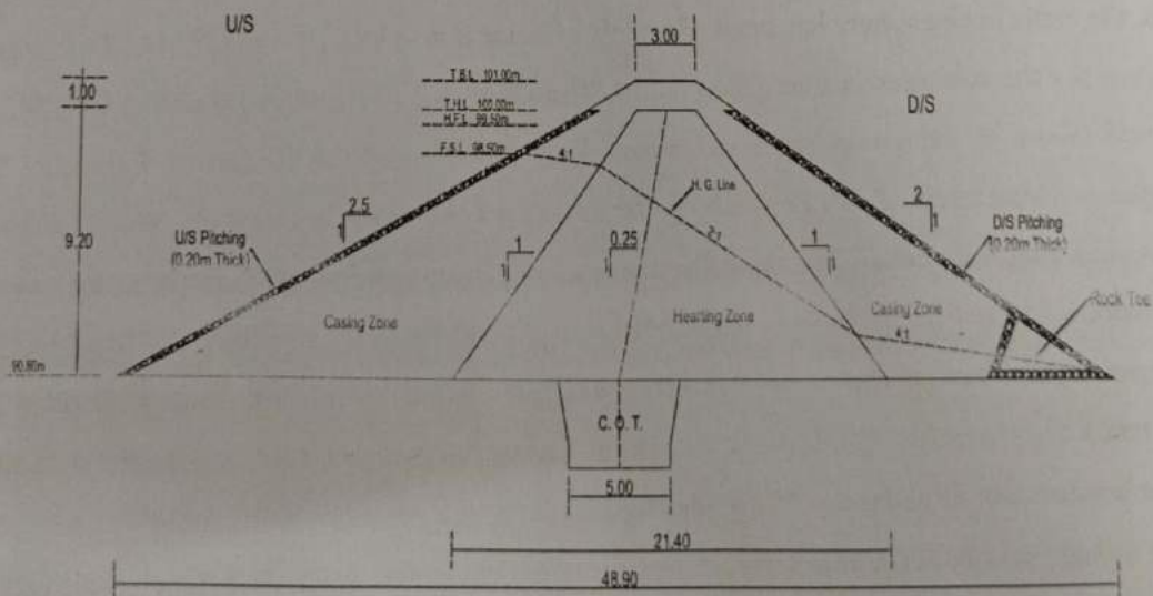
Typical C/S of Percolation Tank
